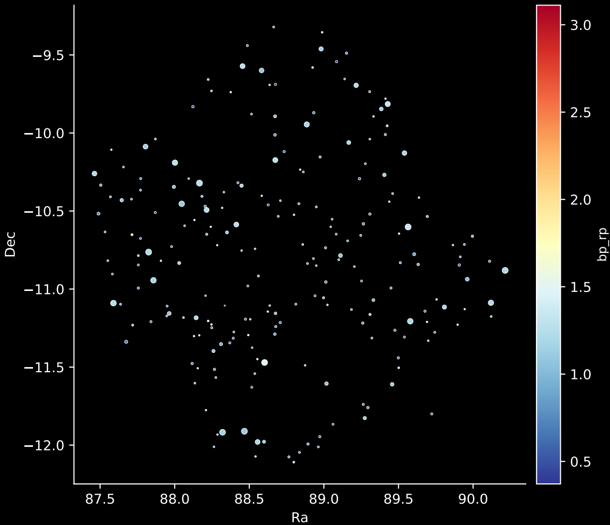
APOGEE DR17 Field: [K2_C12_064-62_btx] Stars: 218
