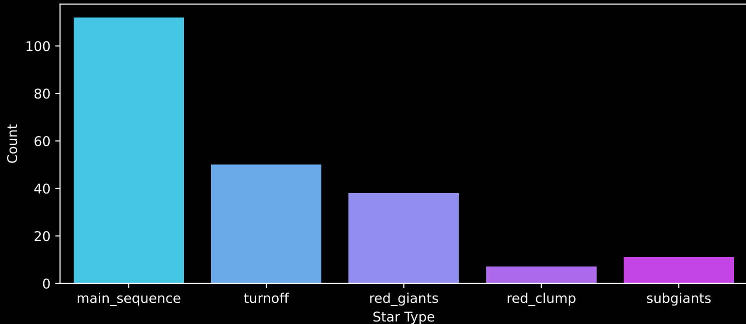
APOGEE DR17 Field: [K2_C12_064-62_btx] Count plot of Star Type
