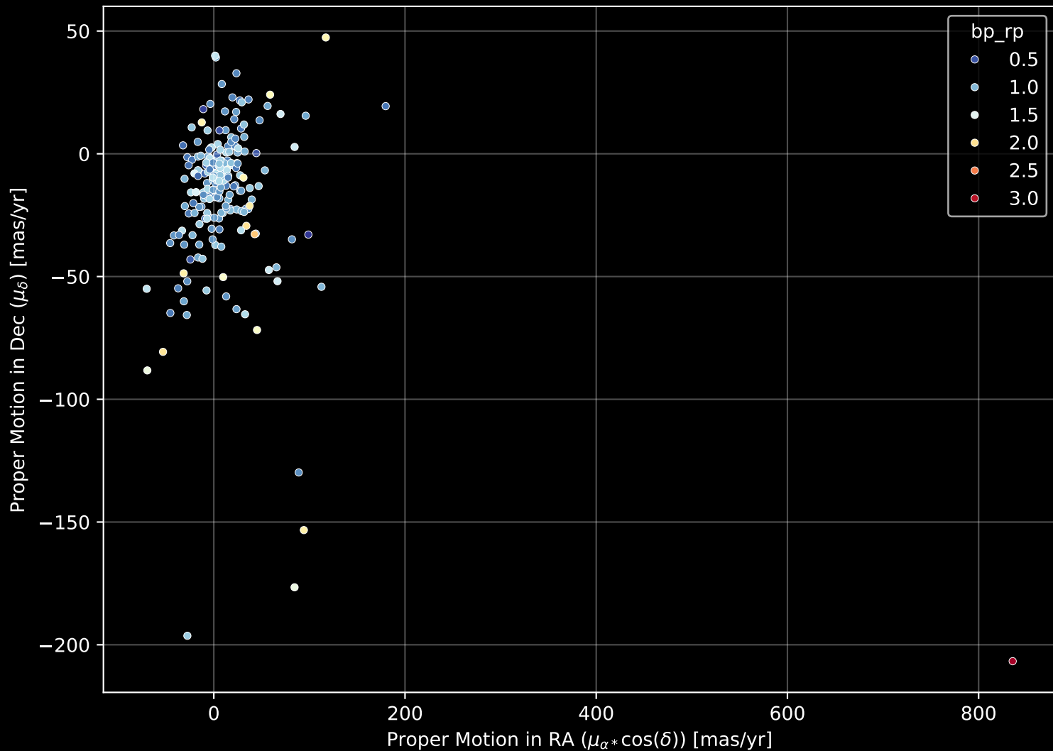
APOGEE DR17 Field: [K2_C12_064-62_btx] Proper Motion Diagram (n= 218)
