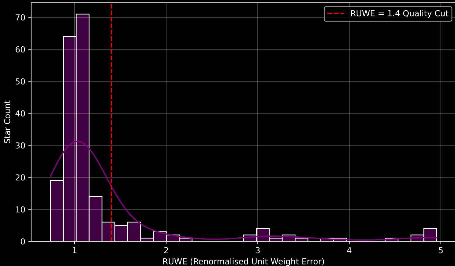
GAPOGEE DR17 Field [K2_C12_064-62_btx] RUWE Distribution (n= 211)
