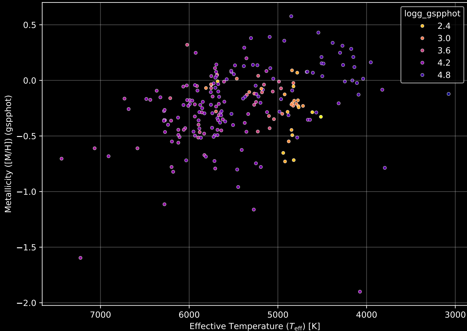
APOGEE DR17 Field: [K2_C12_064-62_btx] Stellar Population Parameters (n= 218)
