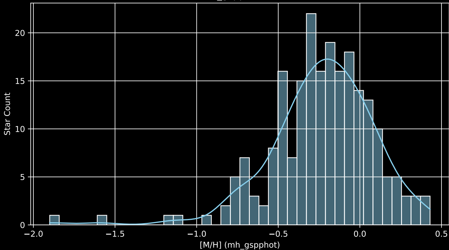
APOGEE DR17 Field: [K2_C12_064-62_btx [M/H] (mh_gspphot) (n= 217)
