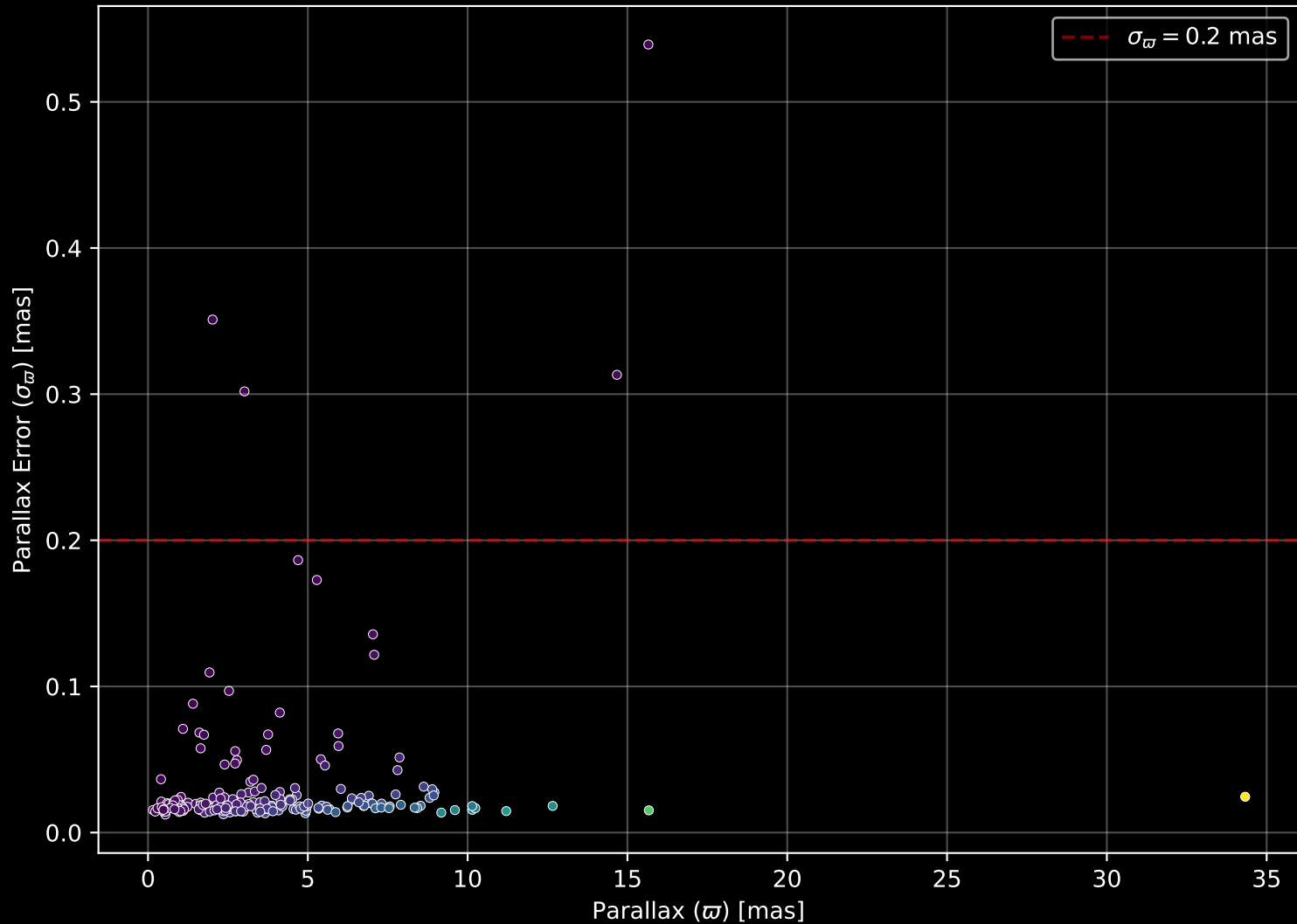
APOGEE DR17 Field: [K2_C12_064-62_btx] Parallax Quality (n= 218)
